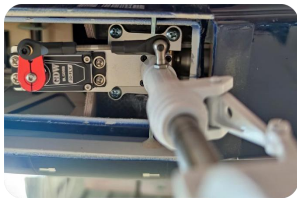
Nose gear
